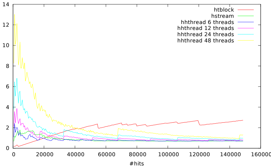
Performance, Mhits/s
