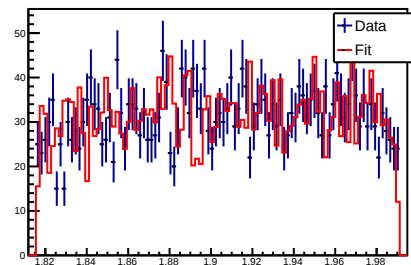
M(XibarpKm)
