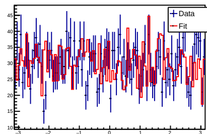
Phi (Km_HeliXibarpLambdaKm)
