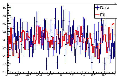
Theta (Km_HeliXibarpLambdaKm)
