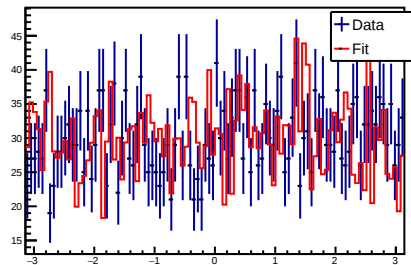
Theta (Xibarp_HeliXibarpLambdaKm)
