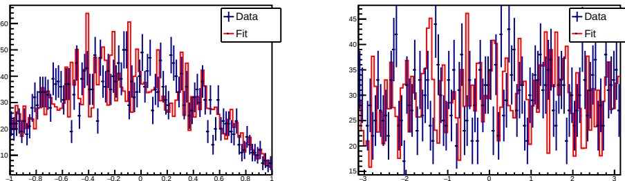
\cos\Theta(\text{Xibar}+_H\text{eliXibar}+\text{LambdaK-}) (fit)
