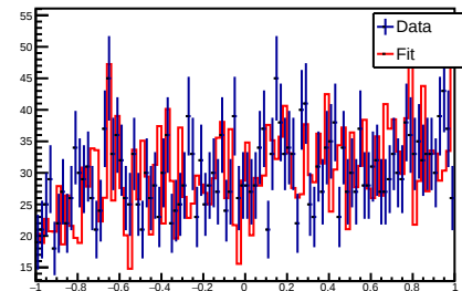
\cos\Theta(\text{Lambda}_H\text{eliXibar}+\text{LambdaK-}) (fit)
