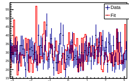
\phi(\text{K-}_H\text{eliXibar}+\text{LambdaK-}) (fit)
