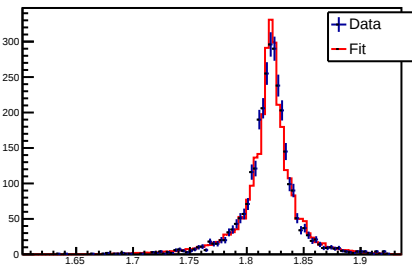
M(\text{LambdaK-}) (fit)
