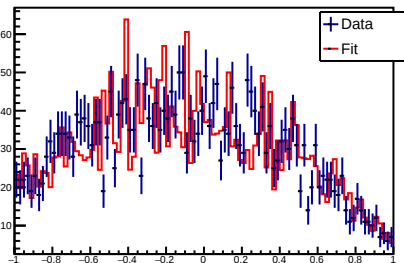
\cos\Theta(\text{Xibar}+_H\text{eliXibar}+\text{LambdaK-}) (fit)
