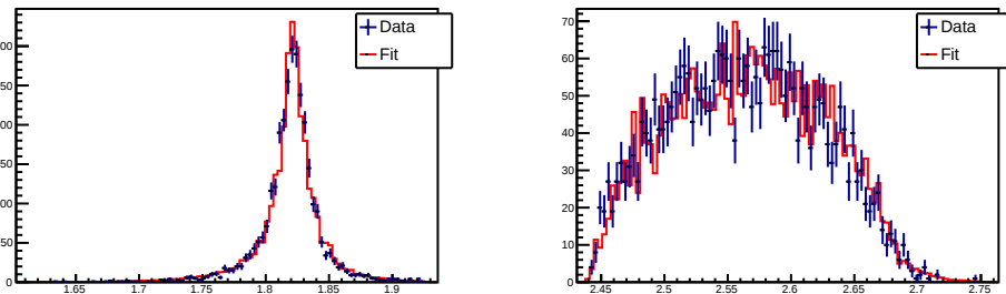
M(\text{LambdaK-}) (fit)
