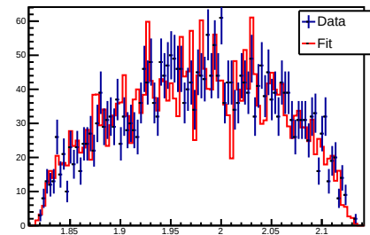
M(\text{Xibar}+\text{K-}) (fit)
