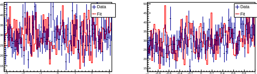
\phi(\text{Lambda}_H\text{eliXibar}+\text{LambdaK-}) (fit)
