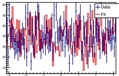
\phi(\text{Lambda}_H\text{eliXibar}+\text{LambdaK-}) (fit)
