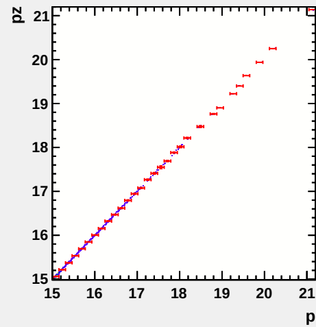
pz versus p (Background)_Id
