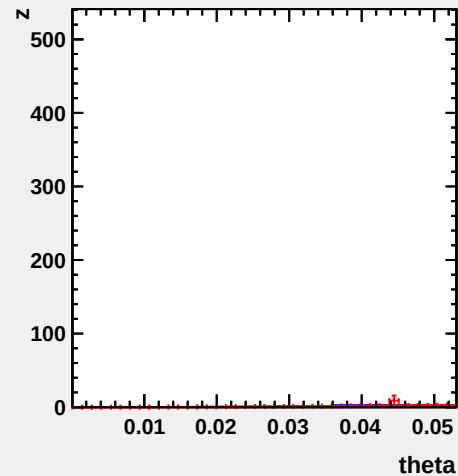
z versus theta (Background)_Id
