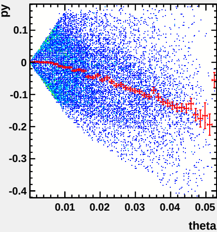
py versus theta (Background)_Id
