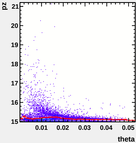
pz versus theta (Background)_Id
