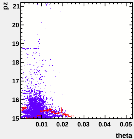
pz versus theta (Signal)_Id
