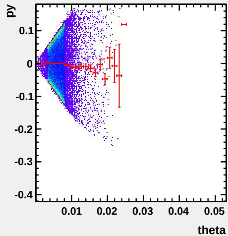
py versus theta (Signal)_Id
